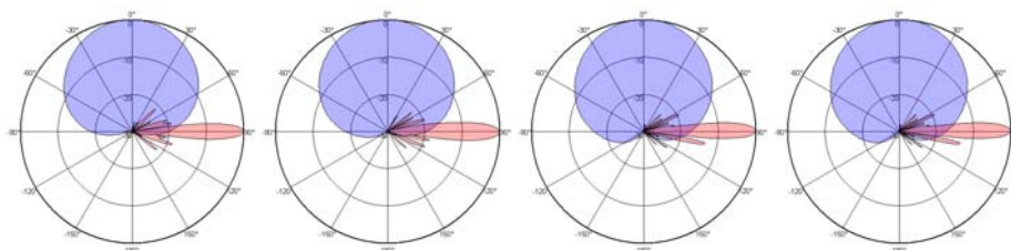
1710~1880 MHz 1920~2200 MHz 2200~2500 MHz 2500~2690 MHz
