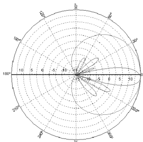
925 MHz
