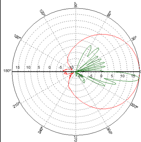
Typical Horizontal and Vertical 7228.06 Patterns
