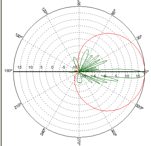
Typical Horizontal and Vertical 7218.19 Patterns
