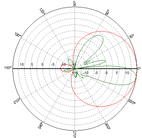
Typical Horizontal and Vertical 7217.11 Patterns
